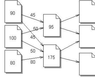
Figure 4. An example of simplified version of PageRank
